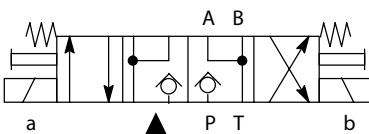
DG4VP-3-105C
