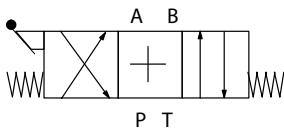
DG17V4-01**-10 Lever operator
