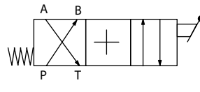
DG17V4-01*AL-10
