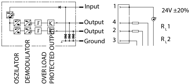
Electrical schematic and mating connector detail I
