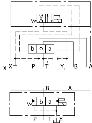
Spring offset, end-to-end, opposite hand, DG5V-7*AL
