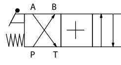
DG17V4-01*AL-10
