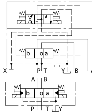
Detented, DG5V-8-*N
